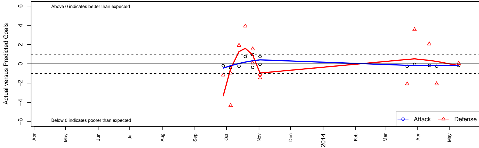
Pendleton Talbot B99 Dots are actual minus expected GF (blue circles) and GA (red triangles). Blue line is smoothed change in attack strength. Red is smoothed change in defense strength.
